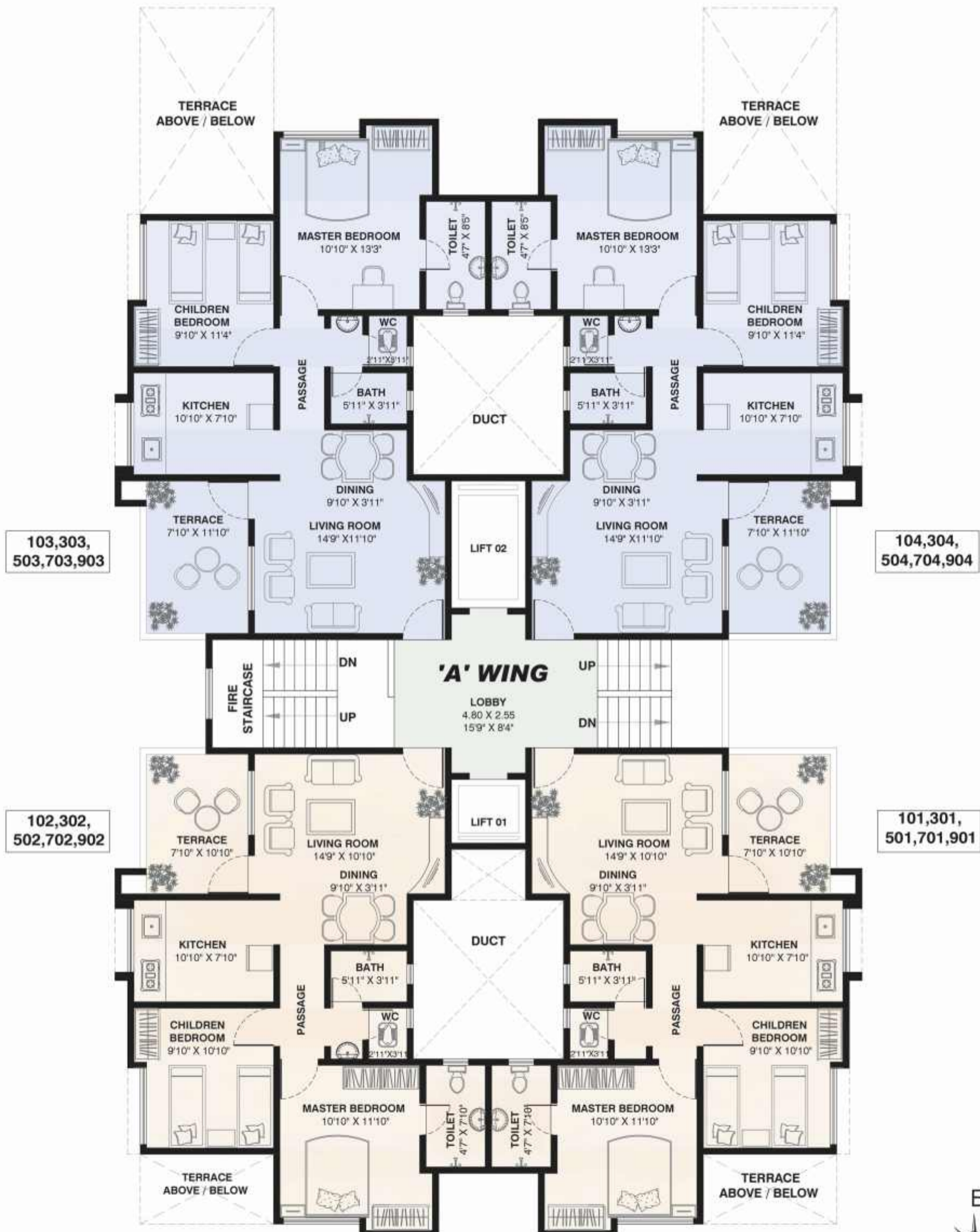
STILT, SECOND, FOURTH, SIXTH & EIGHTH FLOOR PLAN 'A' WING
